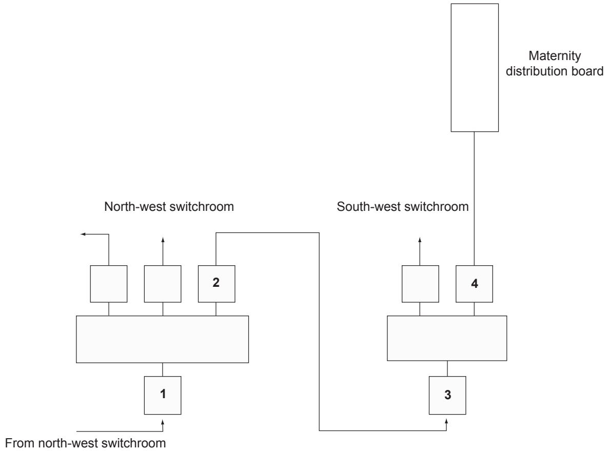
Figure A2 Switchgear network diagram
