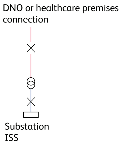
Figure 6 HV Network, one radial circuit, one substation
