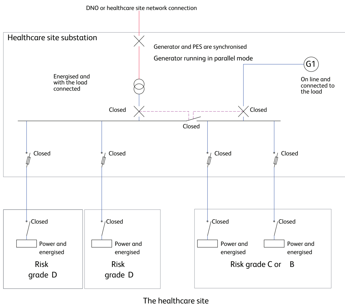
Figure 18 Generator(s) operating in parallel with PES
