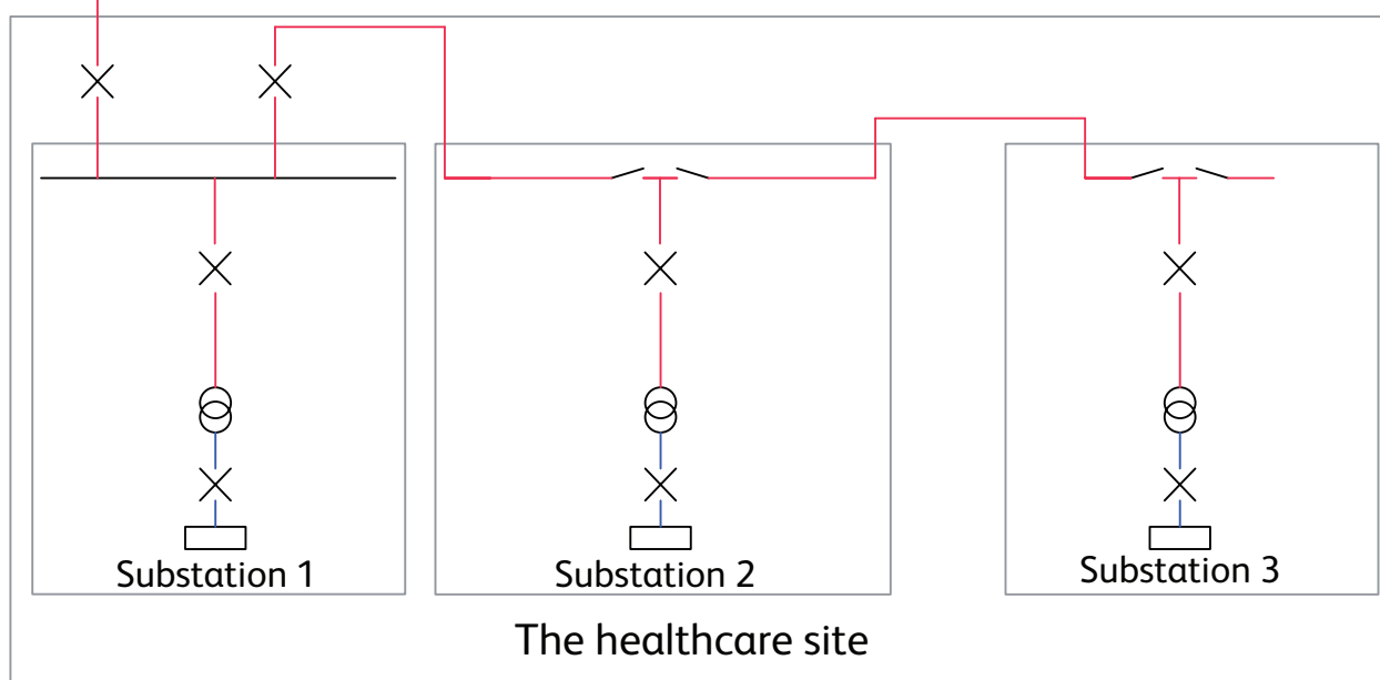
Figure 7 HV Network, one radial circuit, three substations
