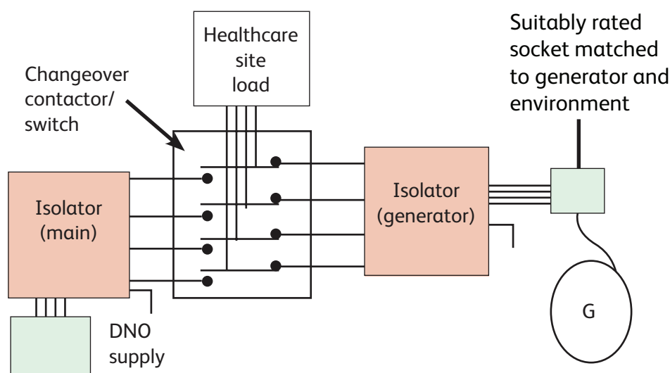
Figure 16 Mobile generator connections
