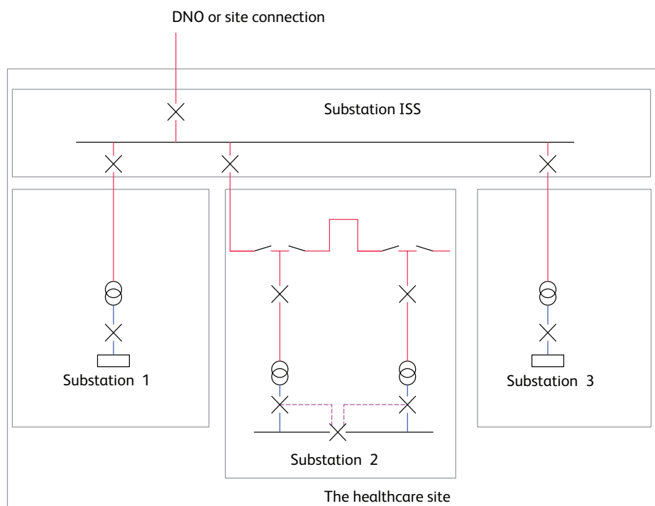
Figure 8 HV network - three radial circuits each with one substation
