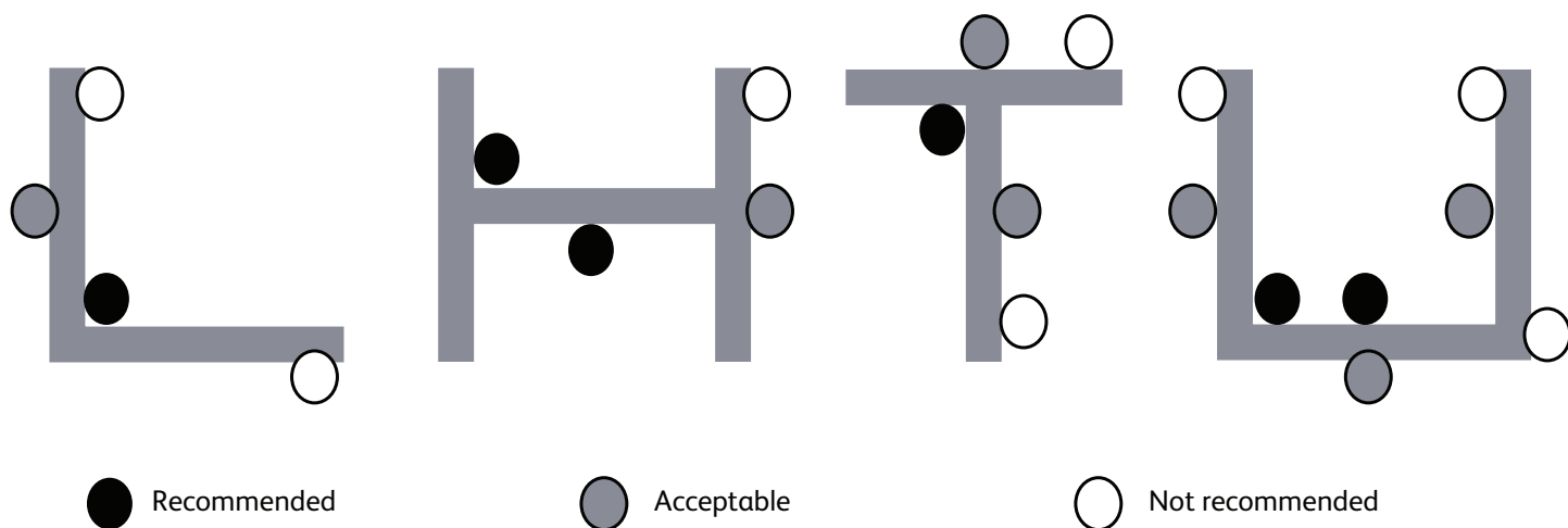
Figure 26 Location of cables inside metallic structural supports
