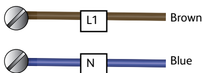
Figure 30 LV single-core cable identification
