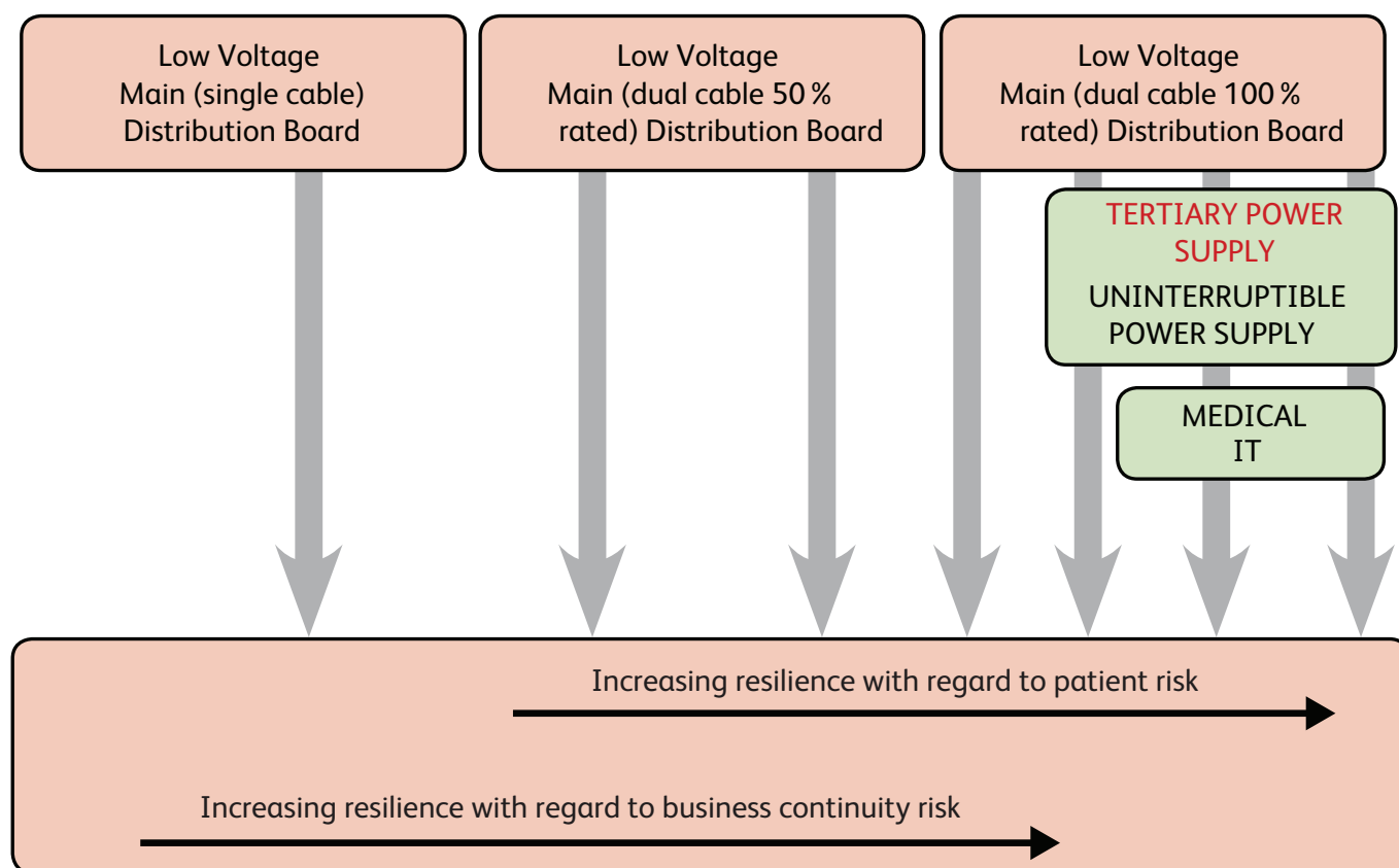
Figure 31 Final-circuit connectivity
