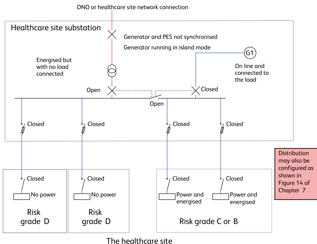
Figure 17 Generator(s) in island operation
