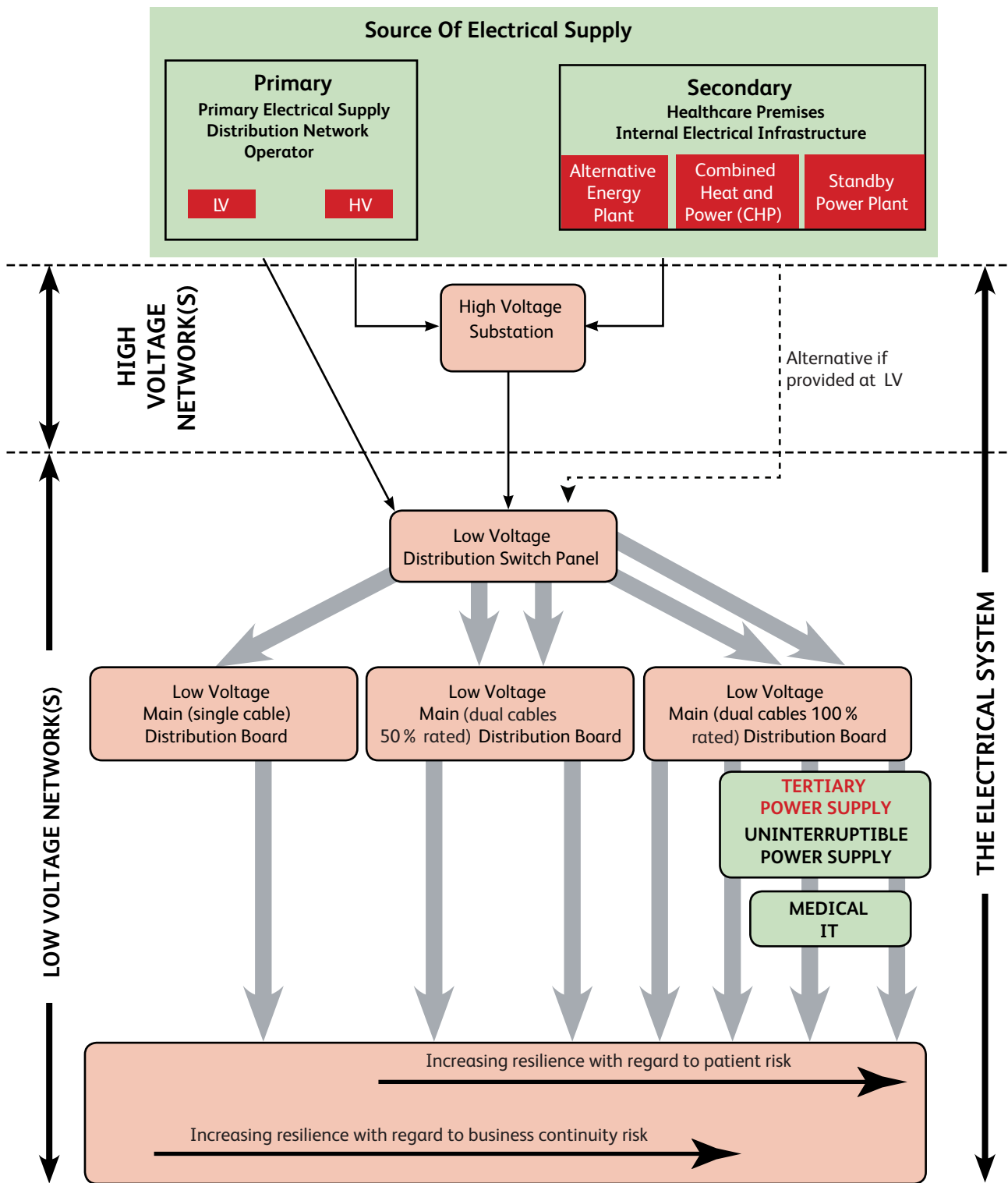
Figure 5 Electrical Infrastructure generic flow diagram
