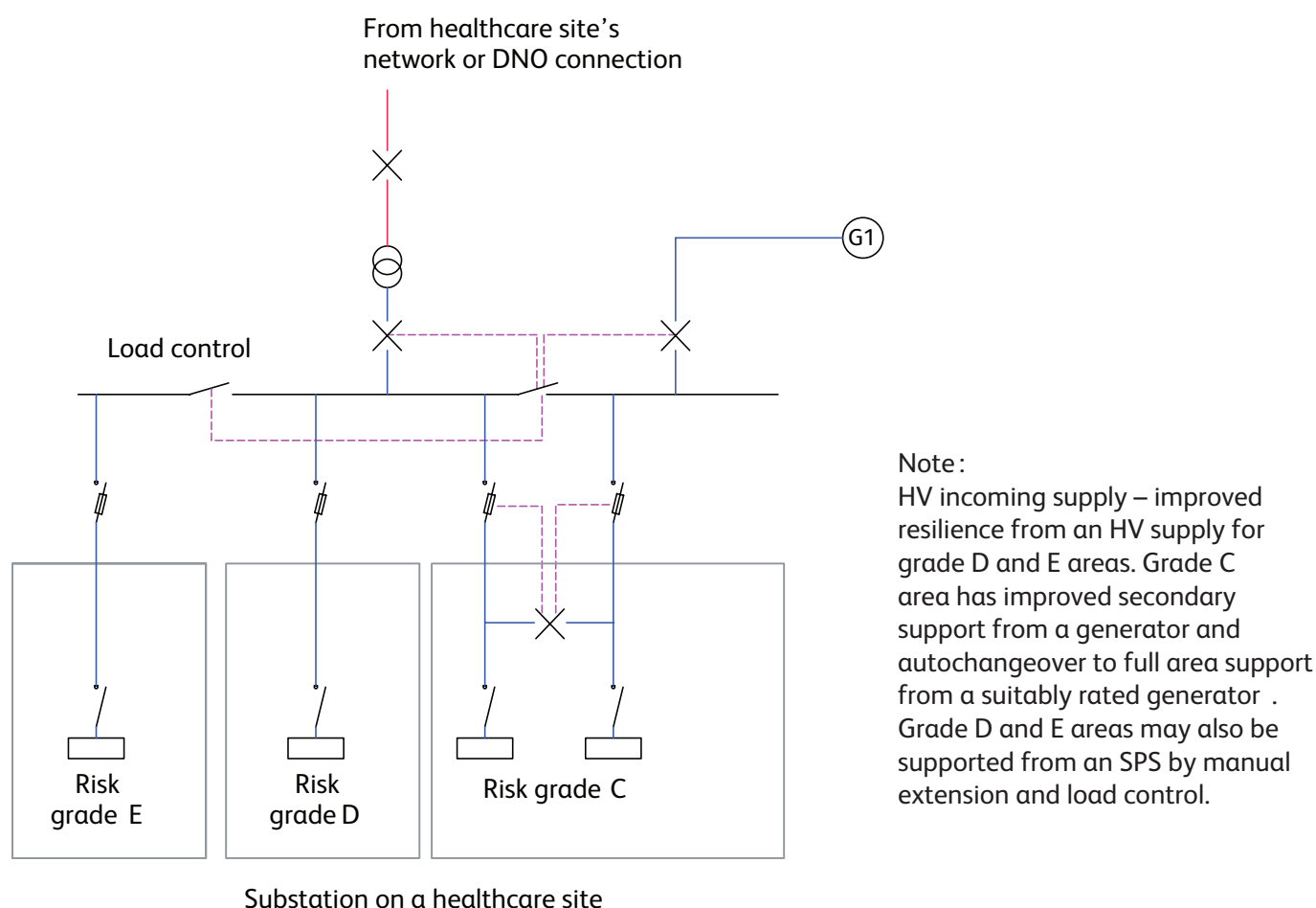
Figure 12 Primary and secondary LV supply - single and dual (100% rated) cable distribution
