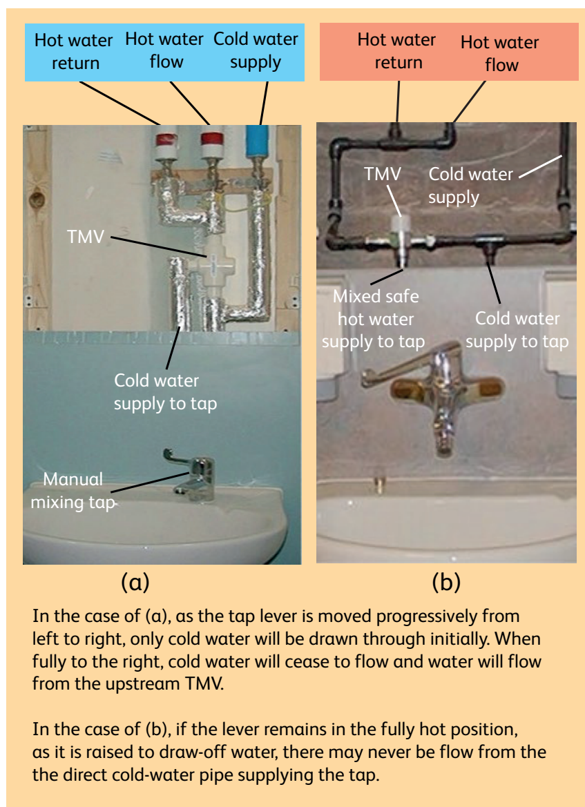
Figure D3 Dead-leg formed by the cold pipework when a TMV is installed upstream of a mixing tap
