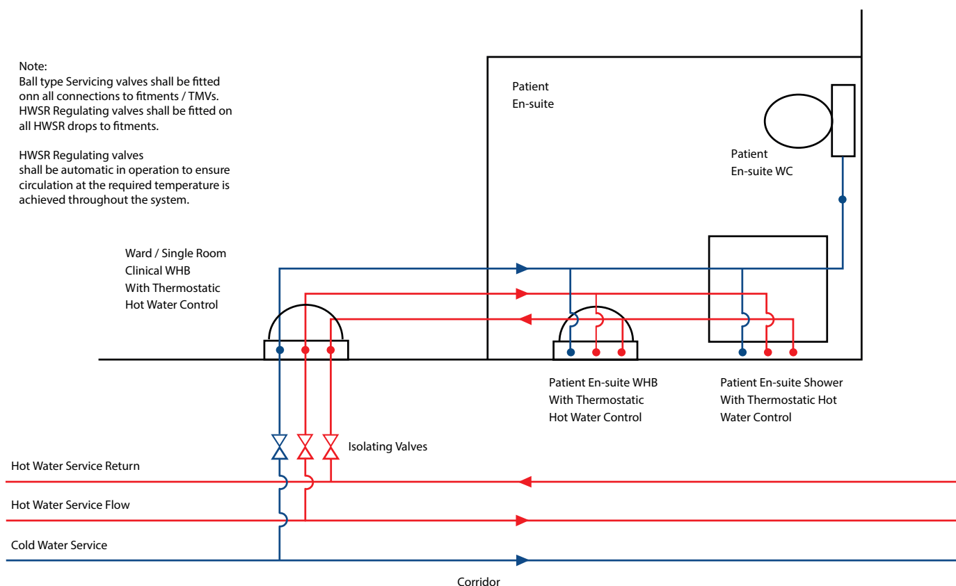
Figure 5 Piping arrangements for an en suite facility
