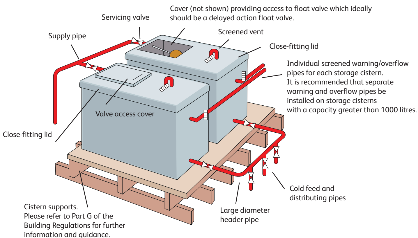
Figure 2 Piping and valve arrangements for dual-cistern installations (Adapted from WRAS 2015)
