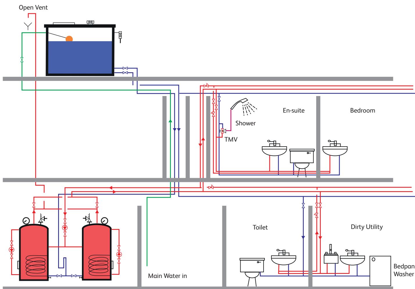
Figure 4 Schematic layout of a cold (and hot) water service system (note: this is a schematic only, and therefore all isolation valves and specific pipework configuration recommendations may not be included)
