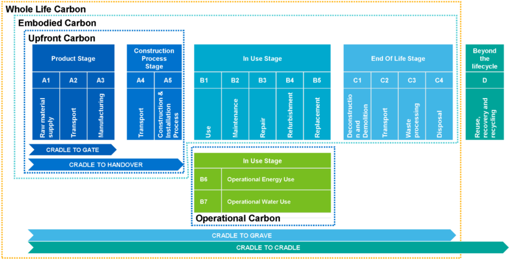
Figure 3.1: Scope of Whole Life Carbon (WLC) based on BS EN 15978
